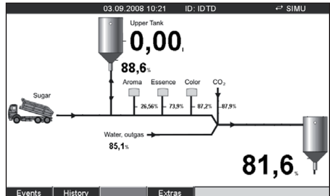
Process display
