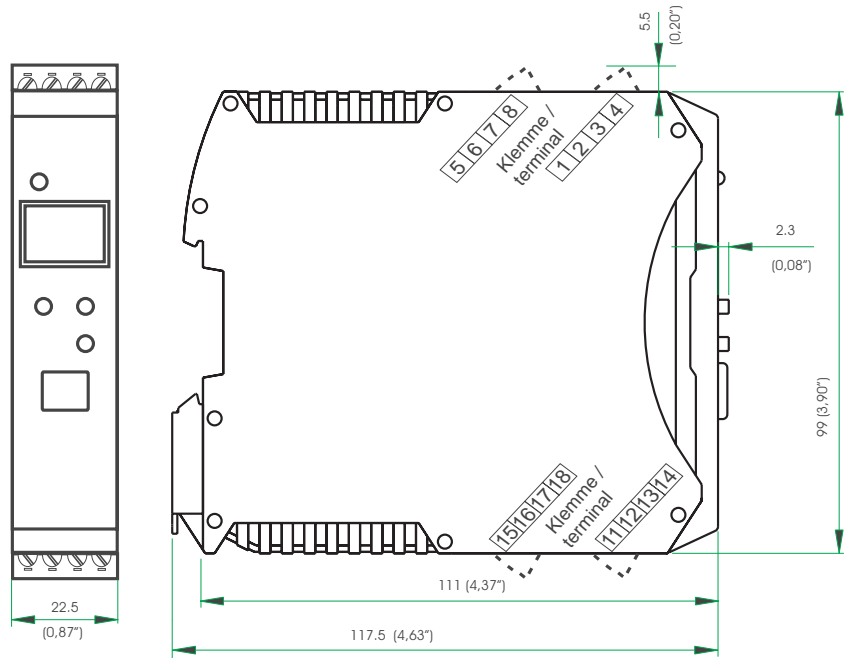
Fig. 4: Dimensions CI 45
